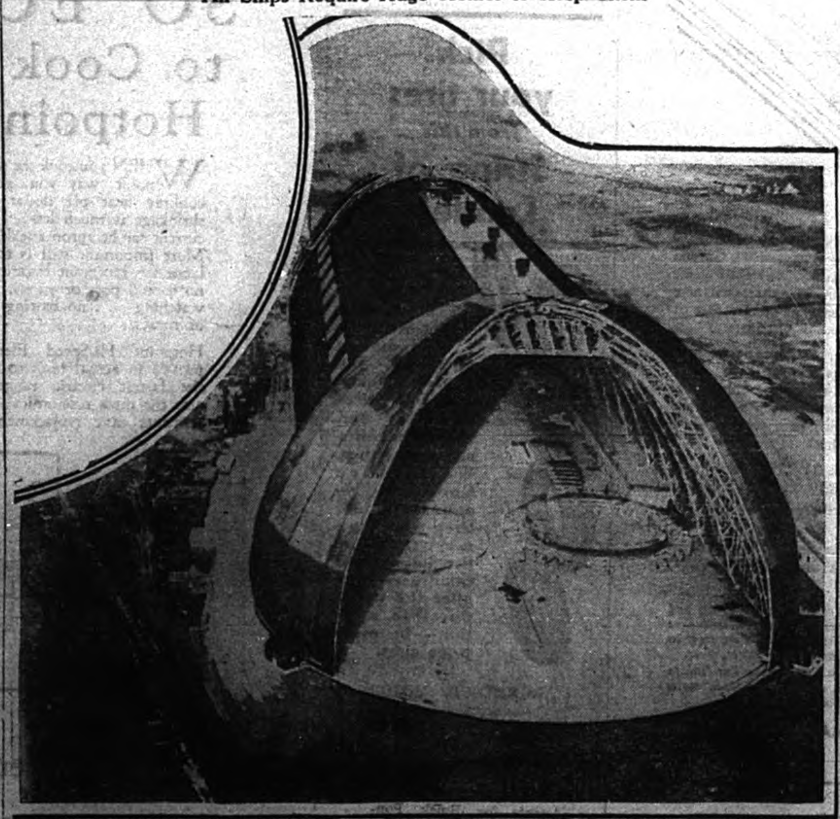
A TYPE OF BUILDING TO BECOME COMMON WITH THE YEARS Aerial view of new Goodyear airship dock at Akron, O. The master ring of the new hangar is nearly completed and will be erected to vertical position in the near future.
