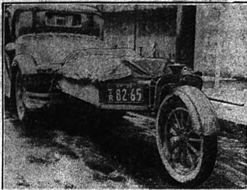
This new type of auto-trailer has only one wheel. It is attached rigidly to rear of automobile, and with its rear wheel shifting as a castor, it is claimed to be easier to manoeuvre than two-wheel trailers.
